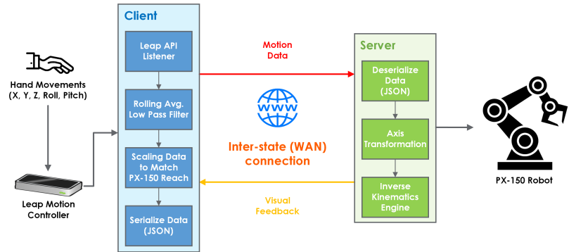
Figure 2: The remote-controlled robotic arm platform.
